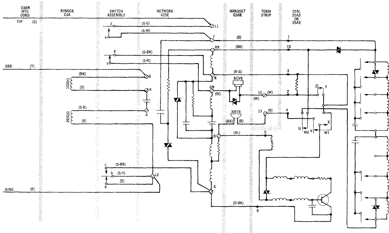
Fig. 3 — 1500D, 2500D, 1554B and 2554B Telephone Sets. Connections With 25A3 or 35A3 Dial. (M.D.)
