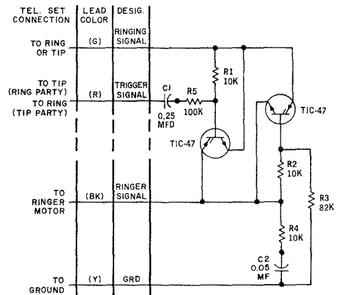
Fig. 2 — Ringer Isolator — Schematic
