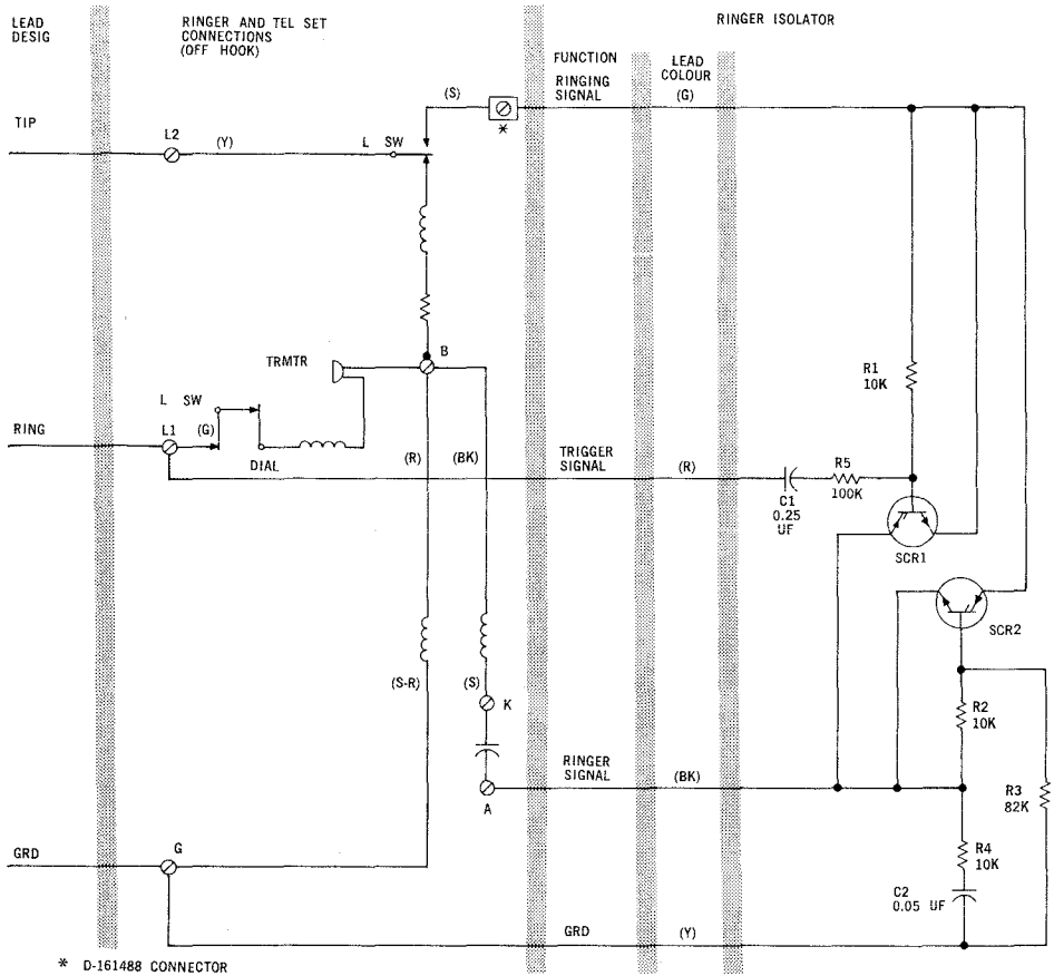
Fig. 4 — Ringer Isolator Connections for Tip Party Identification —2650 Ohms
