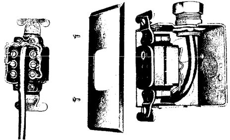
Fig. 7 — 391A Jack Unmounted and 391A Jack Mounted in Outlet Box
