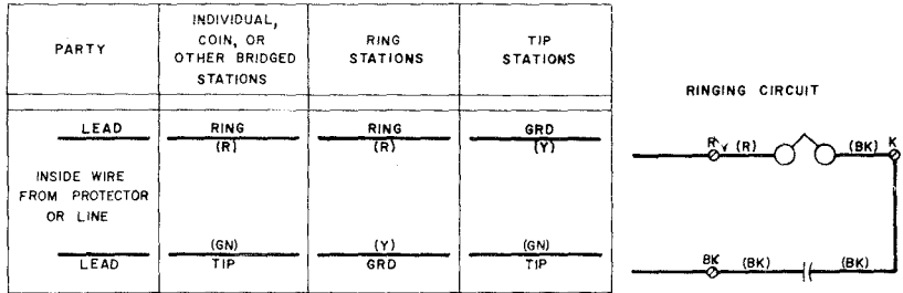
Fig. 1 — 392L and 592A Subscriber Set Connections
