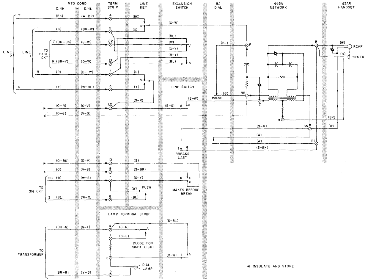
Fig. 1 — 711B Telephone Set — Wired for 2-Line Pickup, Exclusion on Line 1, and Signaling (Used Without 1A1 or 1A2 KTS)
