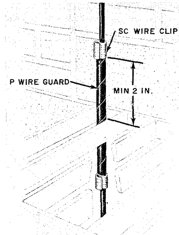
Fig. 5—Protecting Wire Run Through Stationary Metal Grating
