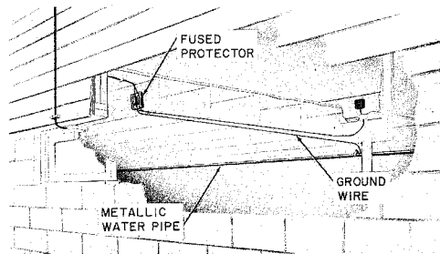
Fig. 20 — Ground Wire Run-Fused Protector
