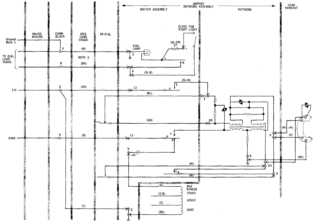
Fig. 1 — 702BQ1A Telephone Set Equipped With QNB442 Network (Early Production) — Connections
