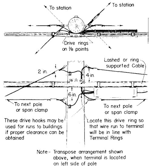
Fig. 1 — Strand Mounted Terminal
