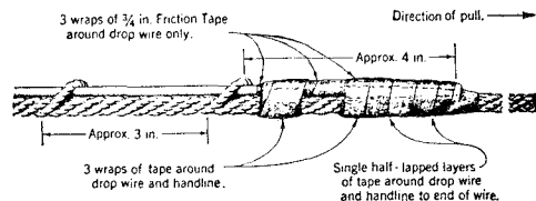
Fig. 4 — Fastening Handline to Prevent Snagging
