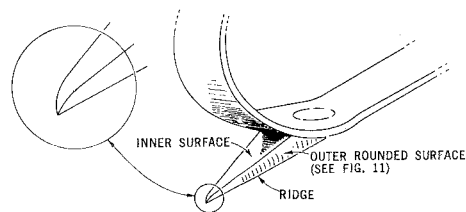
Fig. 10—Gaff Profile and Point
