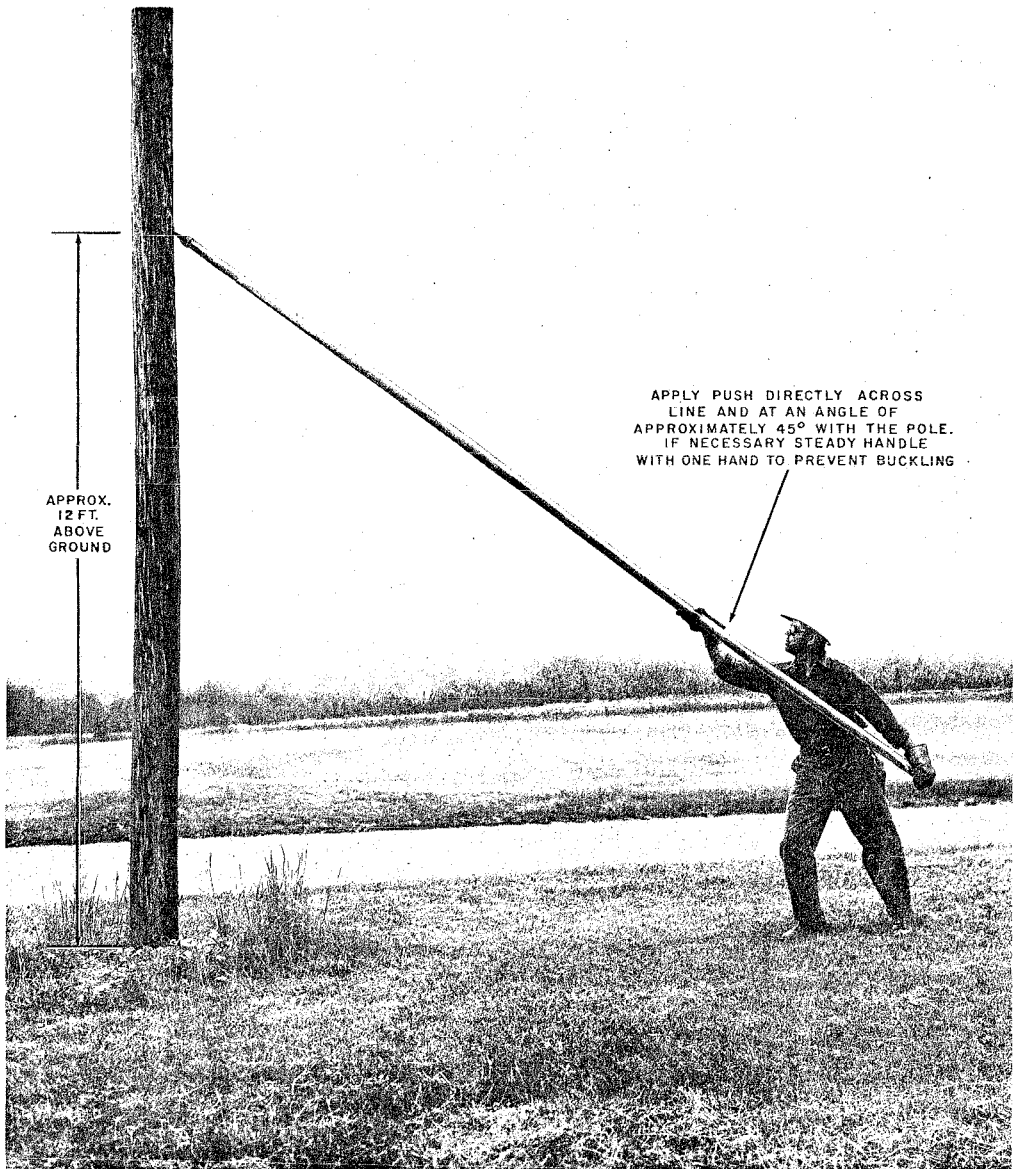
Fig. 1 — Pike Pole Test
