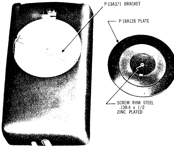
Fig. 19 — 554-Type Housing with 95B Apparatus Blank, Exterior
