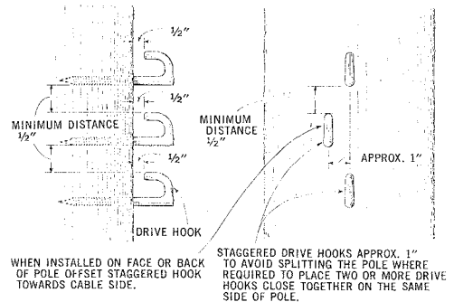
Fig. 1 — Drive Hooks Installed in Pole
