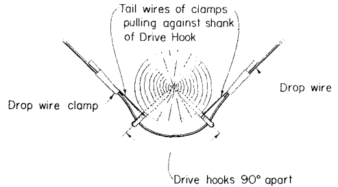
Fig. 6 – Turning Outside Corner
