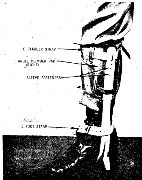
Fig. 9 — Right Climber on Leg
