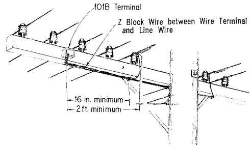
Fig. 14 — Open Wire on Crossarm
