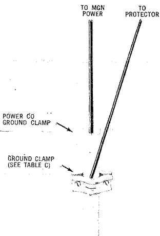
Fig. 34 — MGN Power Grounded to Ground Rod—No Water Pipe—Connection to Pipe Not Possible
