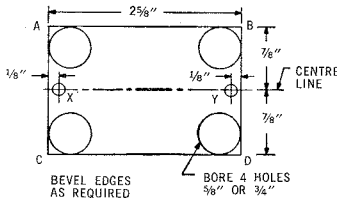
Fig. 5 — Method of Preparing Recess Hole for 391A Jack
