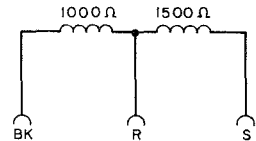
Fig. 2 — Inductor Connections
