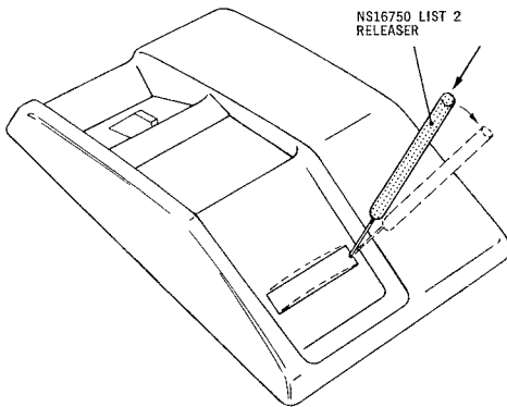
Fig. 6 – Removal of Card Retainer
