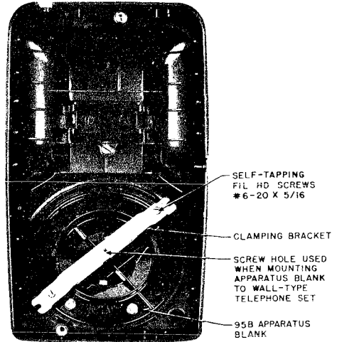
Fig. 18 — 500-Type Housing with 95B Apparatus Blank, Interior
