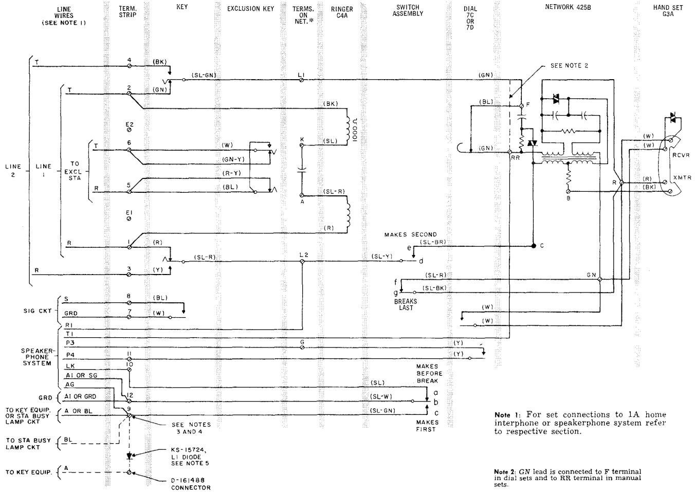
FIG. 2 — 558D TELEPHONE SET (Two-line Pickup, Signaling, Exclusion, and Control Leads)
