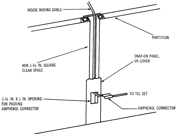
Fig. 17 — Partition Design
