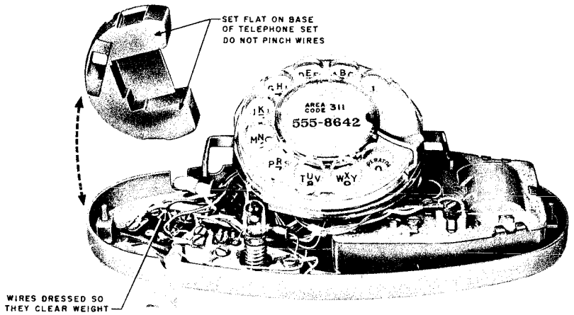
Fig. 16 — P-15E719 Weight Removed from 701B Telephone Set
