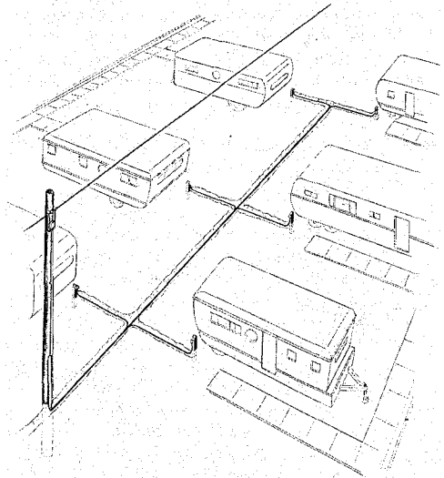
Fig. 2 - Typical Buried Service Connections
