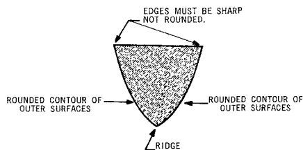
Fig. 11—Outer Surfaces
