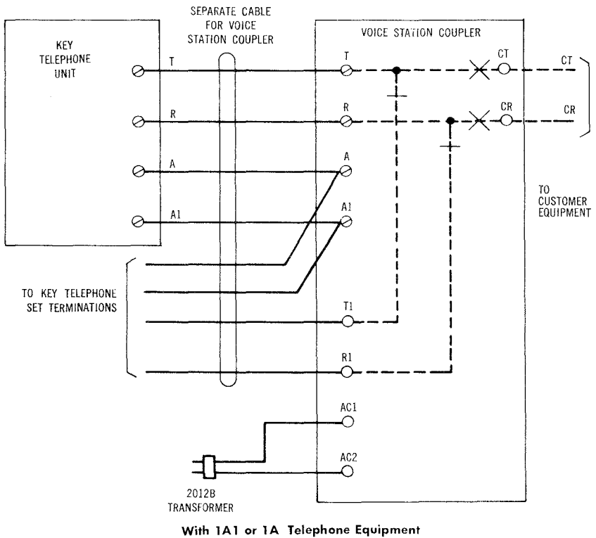
Fig. 5 — "Voice Station Coupler" Electrical Schematic (Associated Recording or Alarm Sending Equipment is provided by the Customer)
