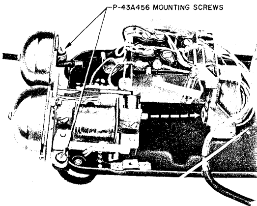
Fig. 21 — 500-Type Set, Ringer Assembly
