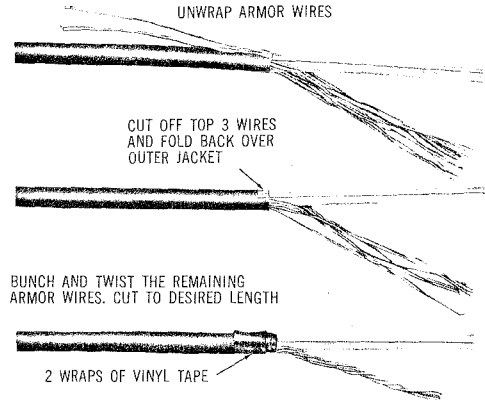
Fig. 1—Preparation of the Armor Wire
