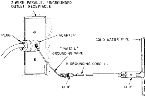
Fig. 8 – Grounding Pigtail
