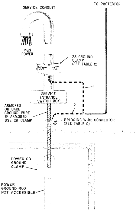
Fig. 35 — MGN Power Grounded to Inaccessible Ground Rod—No Water Pipe—Connection to Pipe Not Possible
