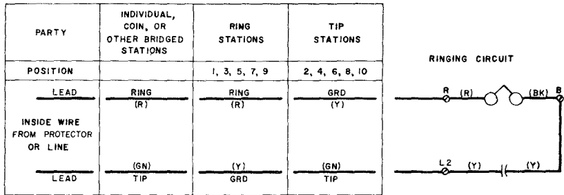
Fig. 2—584DX Subscriber Set Connections
