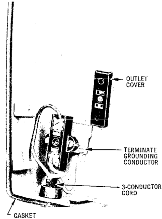
Fig. 2 — Power Cord Termination
