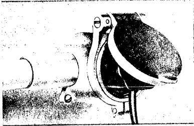
Fig. 17 — Typical Installation of KS-16151 Jack Installed on 1/2-inch Conduit
