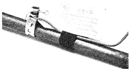
Fig. 21 — Station Ground Clamp Installation
