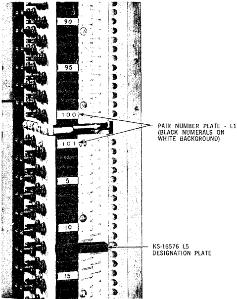
Fig. 45 — KS-16576, L5 Coloured Designation Plate (Red) Installed on 300 Type Connector
